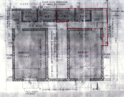
BARSATI FLOOR PLAN
