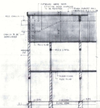
SECTION AT AB
